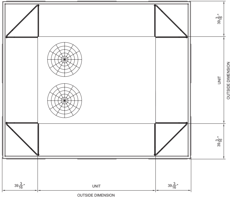
35" VERTICAL STYLE ENVISOR FOOTPRINT
