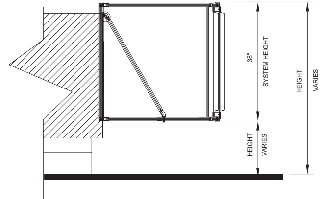
35" VERTICAL STYLE ENVISOR SECTION
