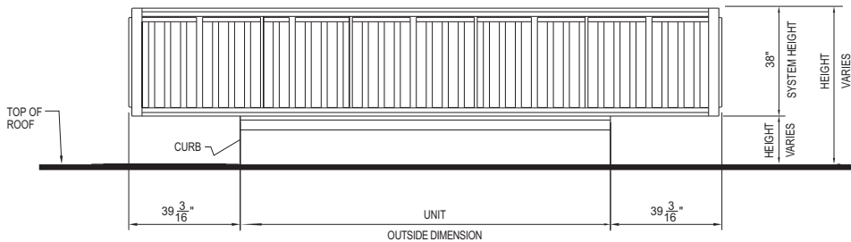
35" VERTICAL STYLE ENVISOR ELEVATION
