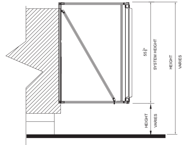
52" VERTICAL STYLE ENVISOR SECTION
