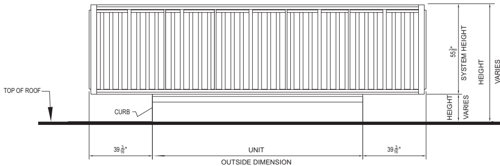
52" VERTICAL STYLE ENVISOR ELEVATION
